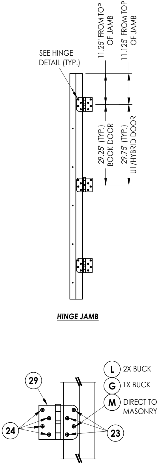
HINGE DETAIL
